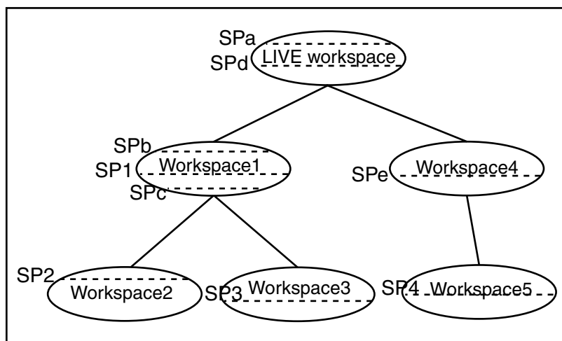
Figure 1–2 Savepoints
